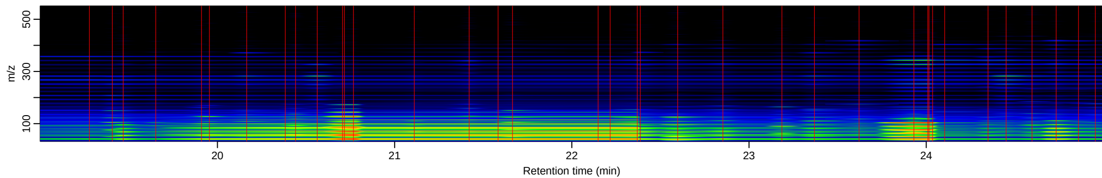
GCMS_data2 | Mean Pearson residual
