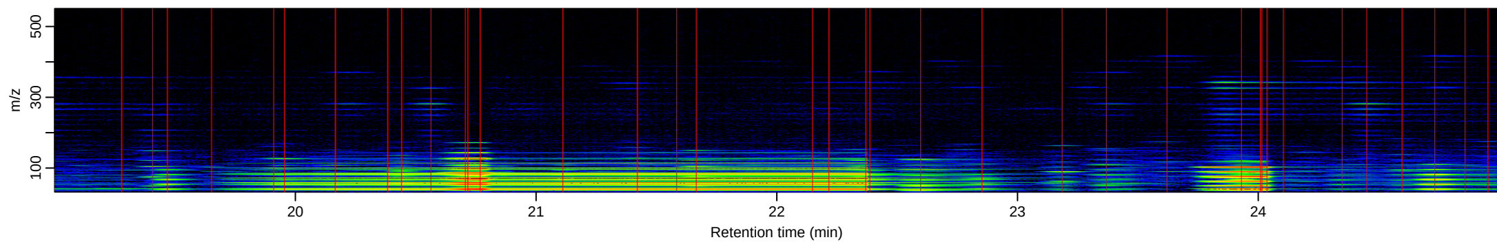
GCMS_data2 | Fitted chromatogram
