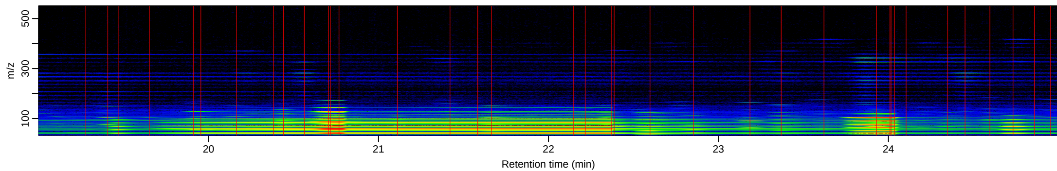
GCMS_data2 | Observed minus modeled background
