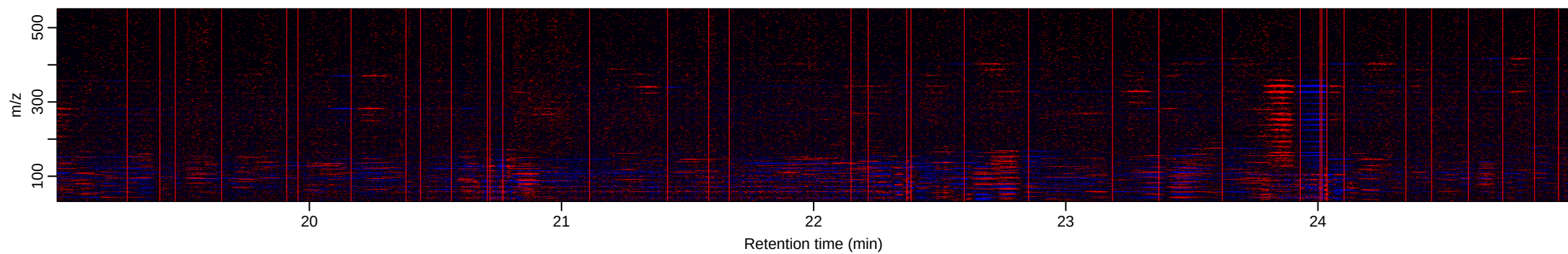
GCMS_data2 | Mean Pearson residual
