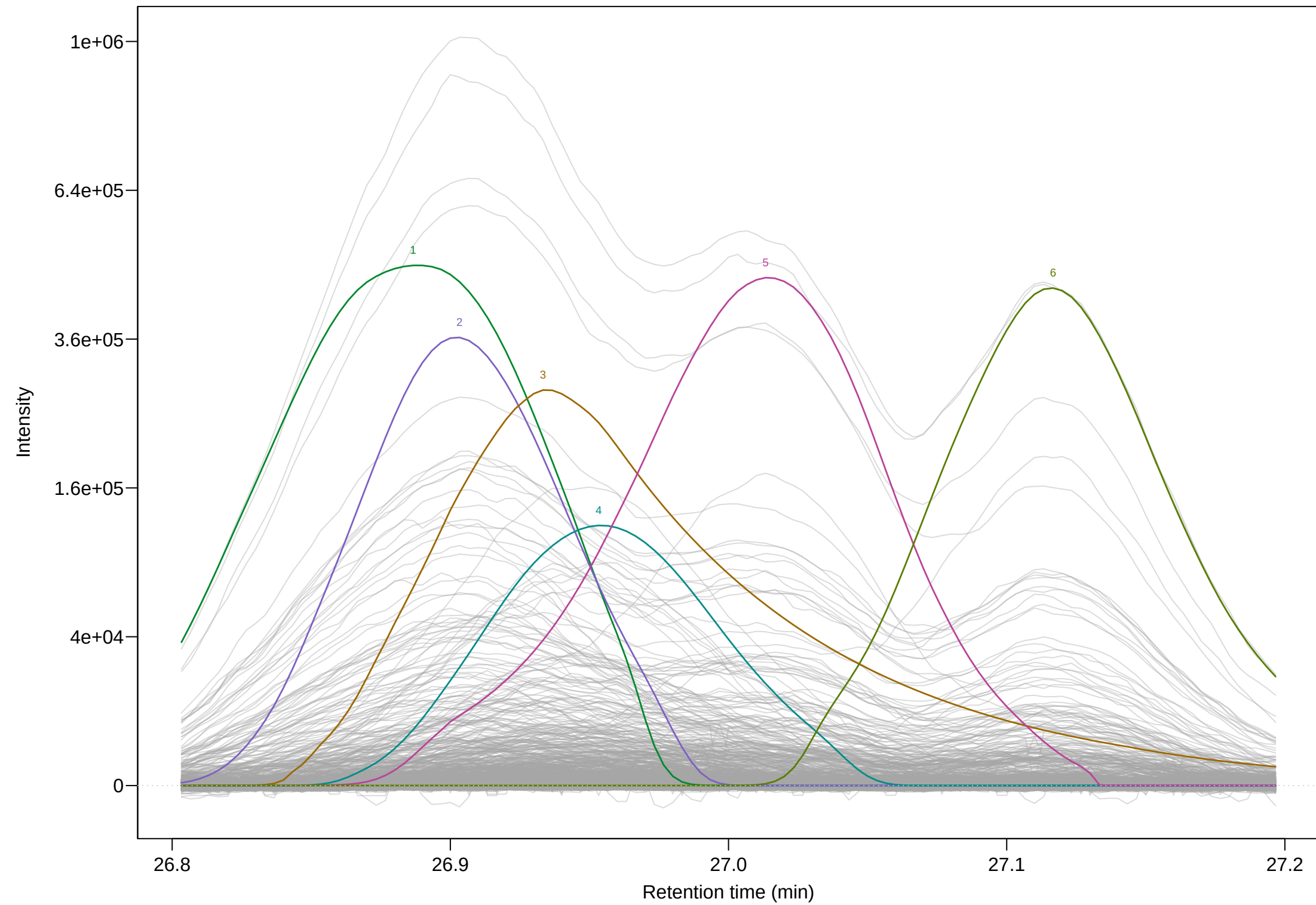
GCMS_data1 | sqrt display | basepeak-scaled compound profiles
