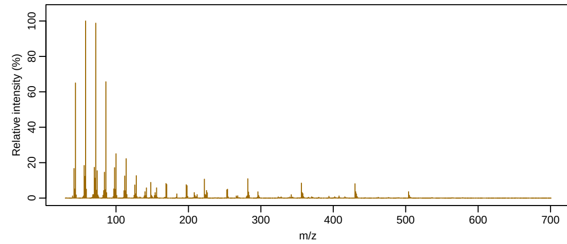
GCMS_data1 | compound 3 | RT 26.933 min
