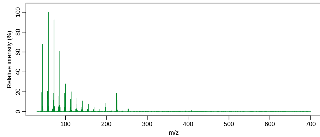
GCMS_data1 | compound 2 | RT 26.903 min
