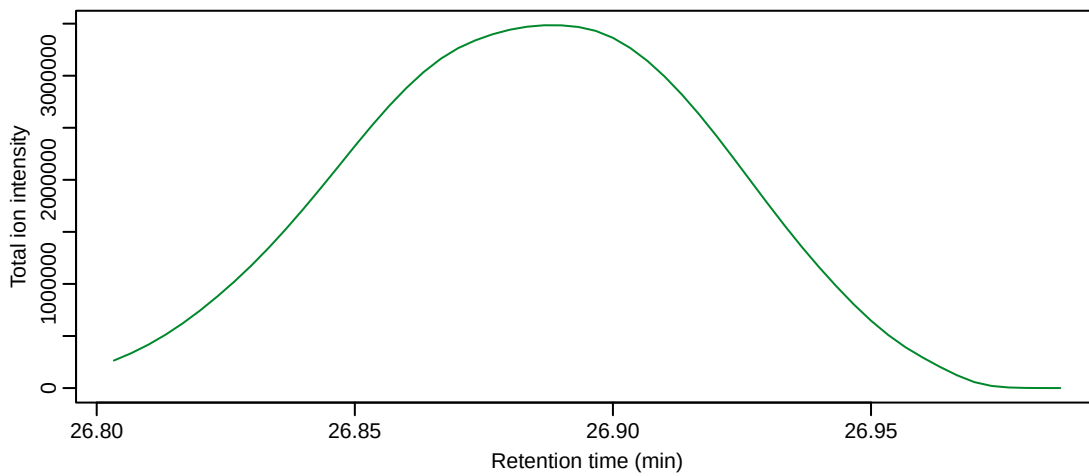
Compound 2 | area 5.165e+07
