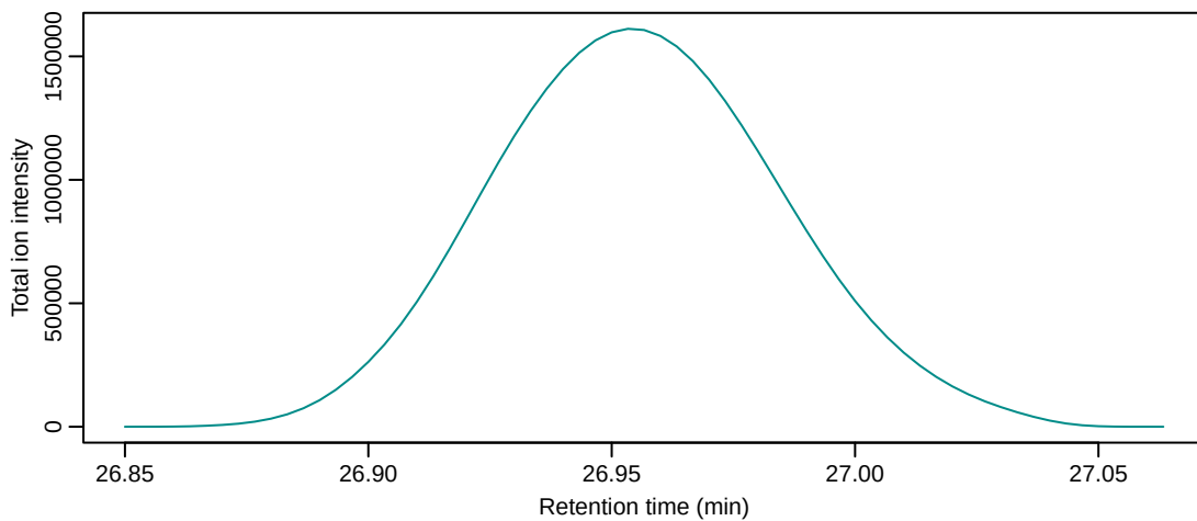
Compound 5 | area 8.077e+07
