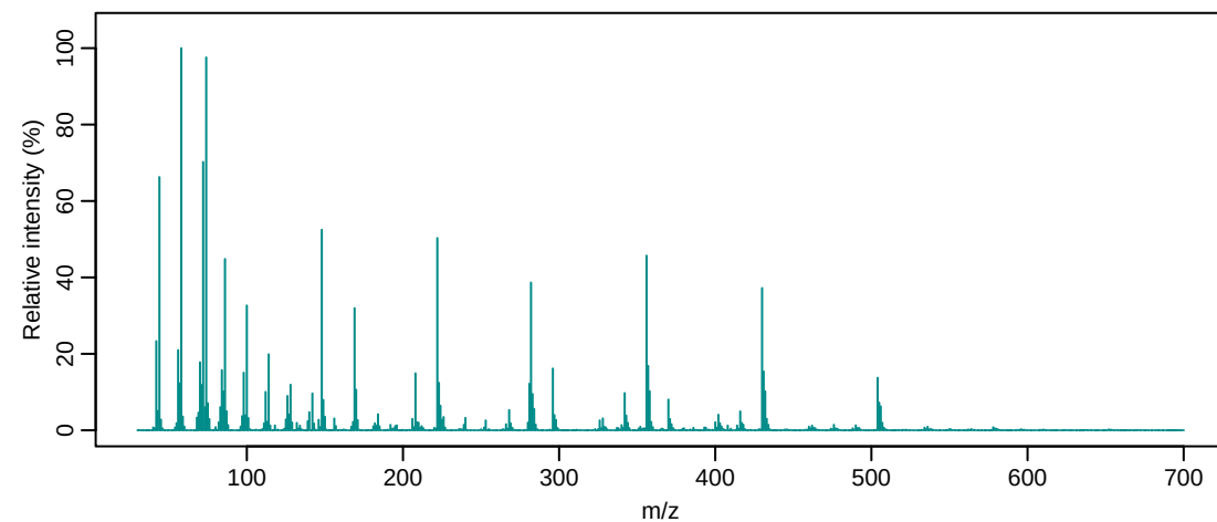
GCMS_data1 | compound 5 | RT 27.013 min
