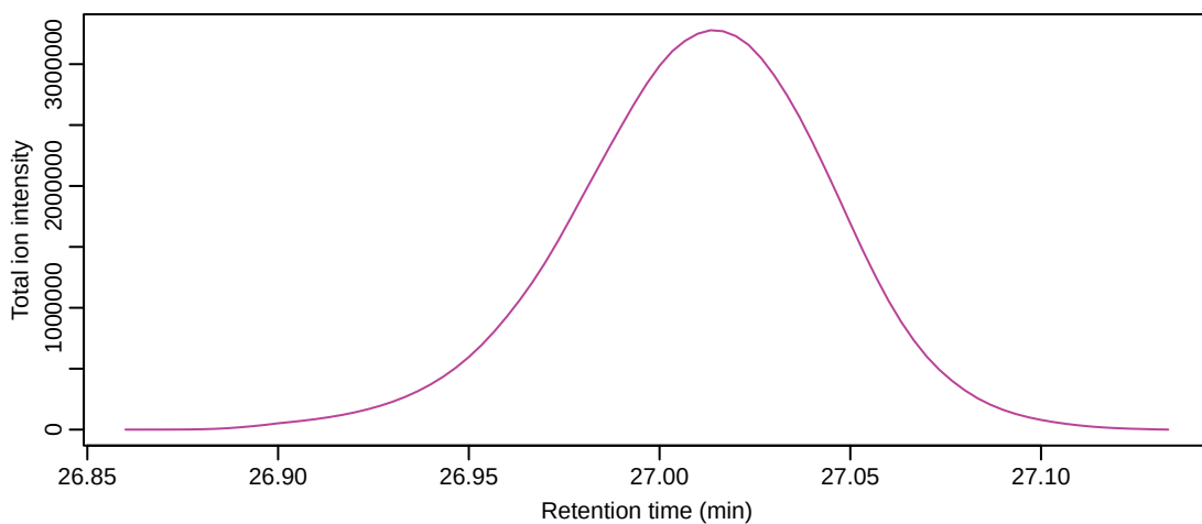
Compound 6 | area 6.119e+07
