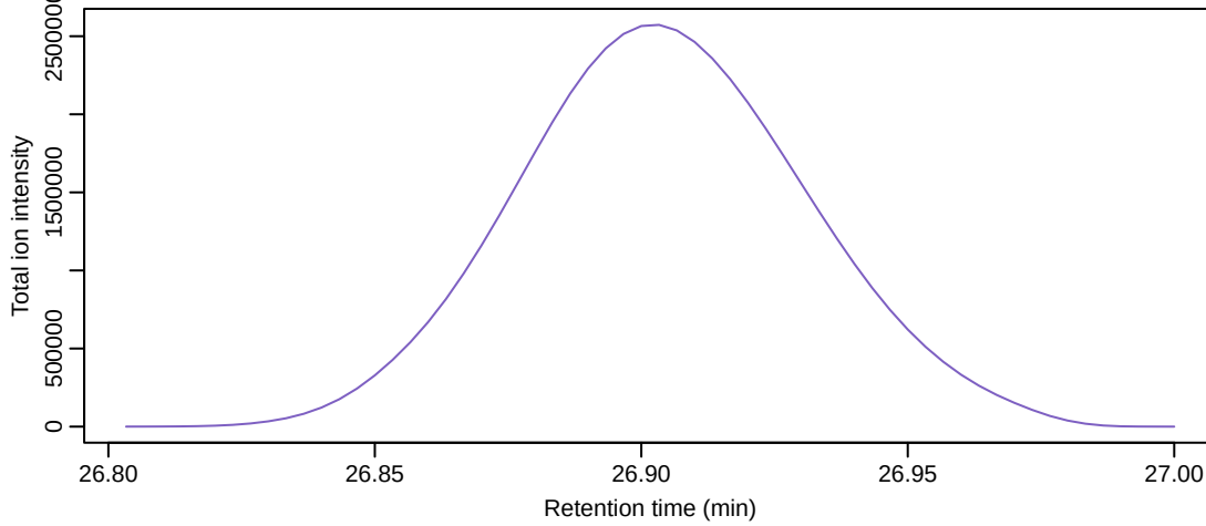
Compound 3 | area 6.064e+07
