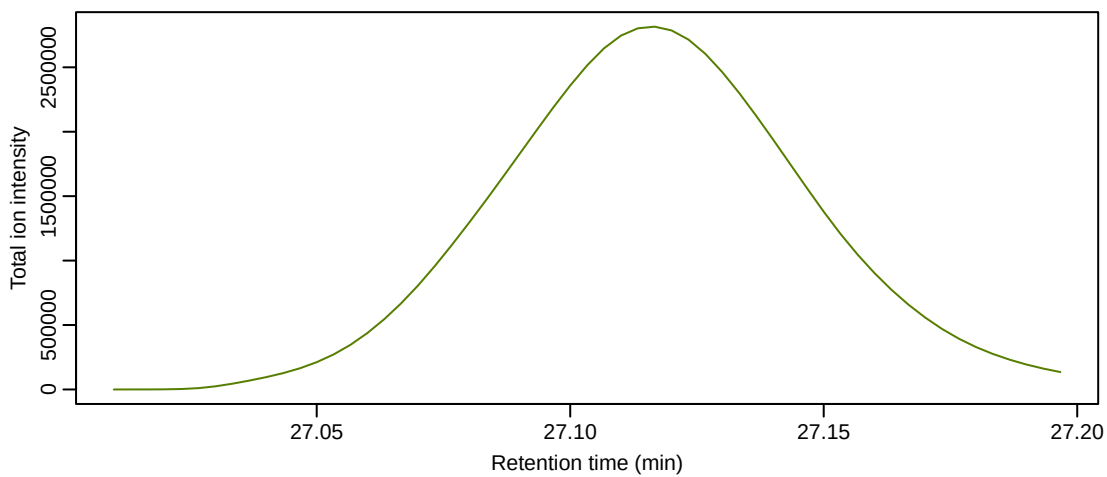
Compound 6 | area 6.119e+07
