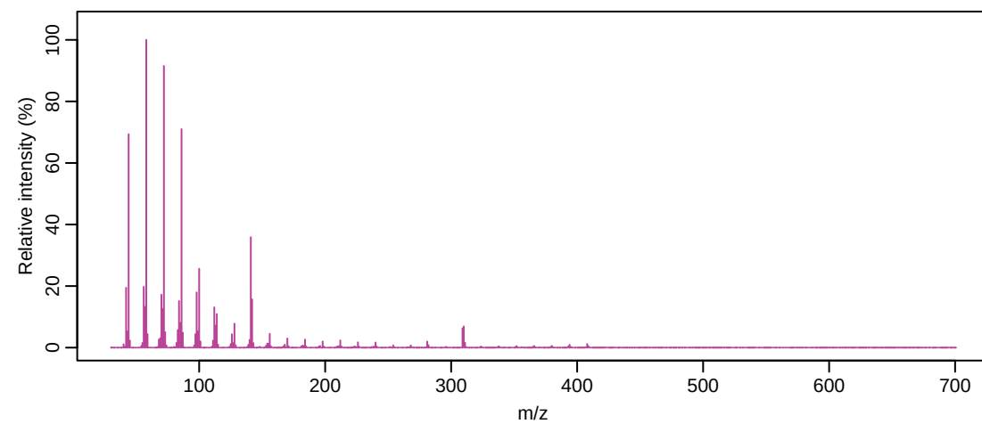
GCMS_data1 | compound 6 | RT 27.117 min
